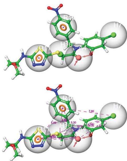
Figure 5: Best Pharmacophoric Hypothesis AHHR_1
